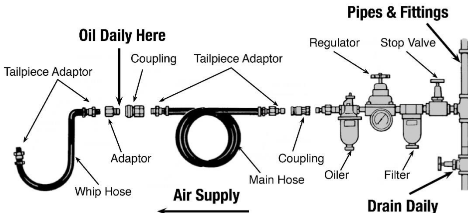
Recommended Air Line Components
